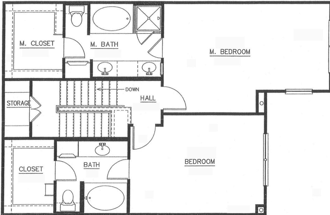
FLOOR PLAN - UFFIZI 2ND FLOOR
